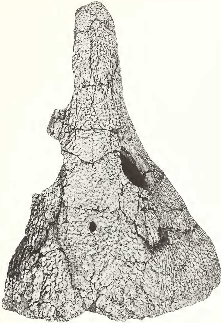
TEXT-FIG. 3. Labidosaurikos meachamii Stovall; Lower Permian; Oklahoma; OMNH 04331, holotype; skull in dorsal view; for interpretation and scale, see Text-figure 2.
